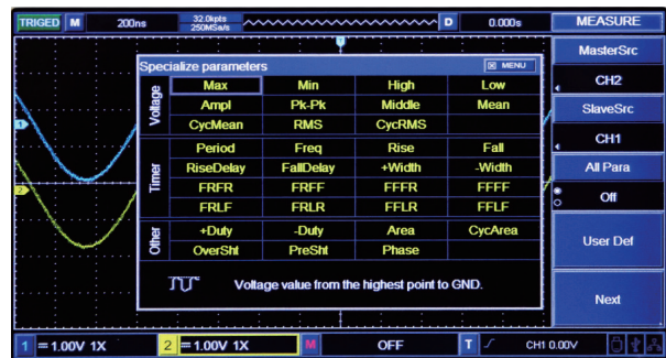
Automatic Measurement of Waveform Parameters
